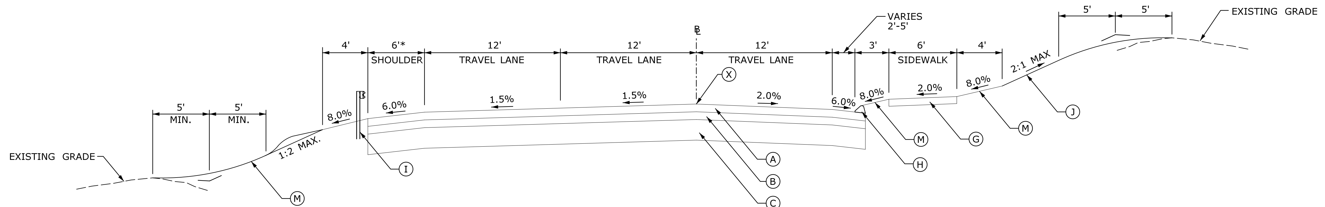
ROUTE 4 FULL DEPTH PAVEMENT CONSTRUCTION TYPICAL SECTION N.T.S.
