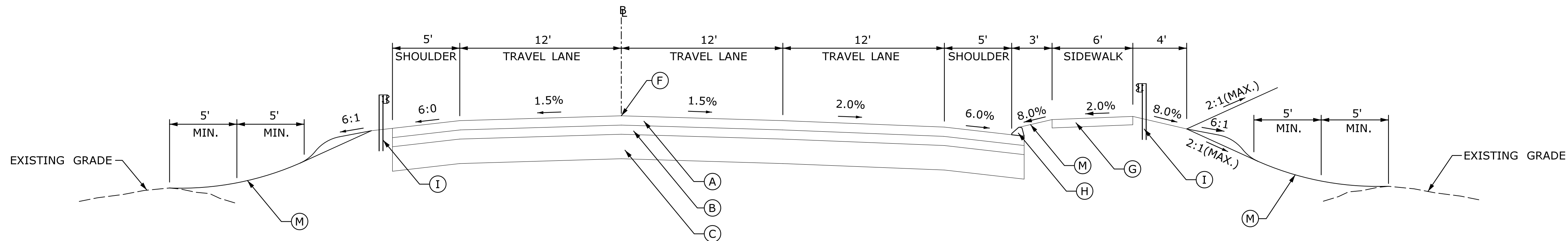
MONTEITH DRIVE EXTENSION FULL DEPTH PAVEMENT CONSTRUCTION TYPICAL SECTION N.T.S.
