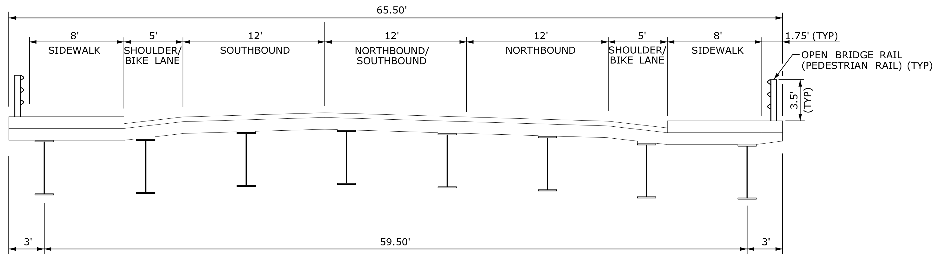
TYPICAL BRIDGE SECTION N.T.S.
