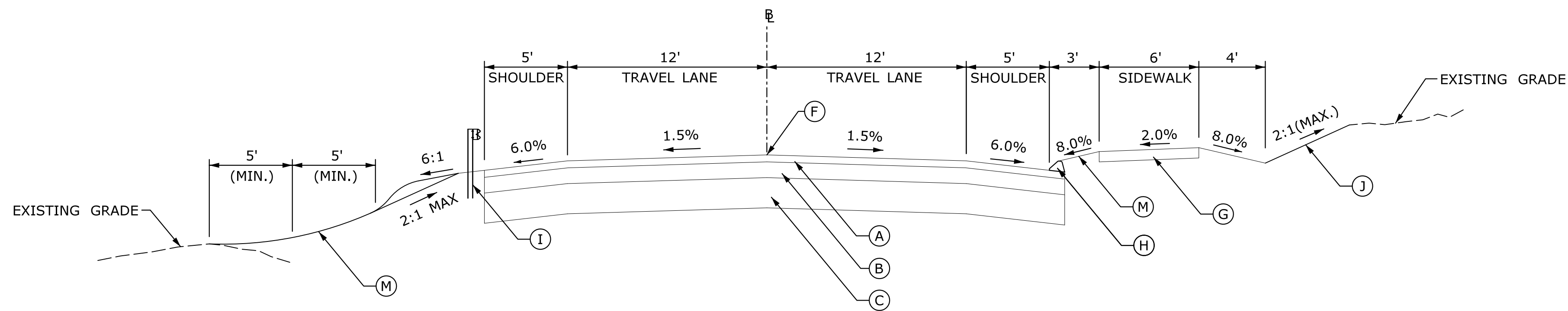
MONTEITH DRIVE EXTENSION FULL DEPTH PAVEMENT CONSTRUCTION TYPICAL SECTION N.T.S.
