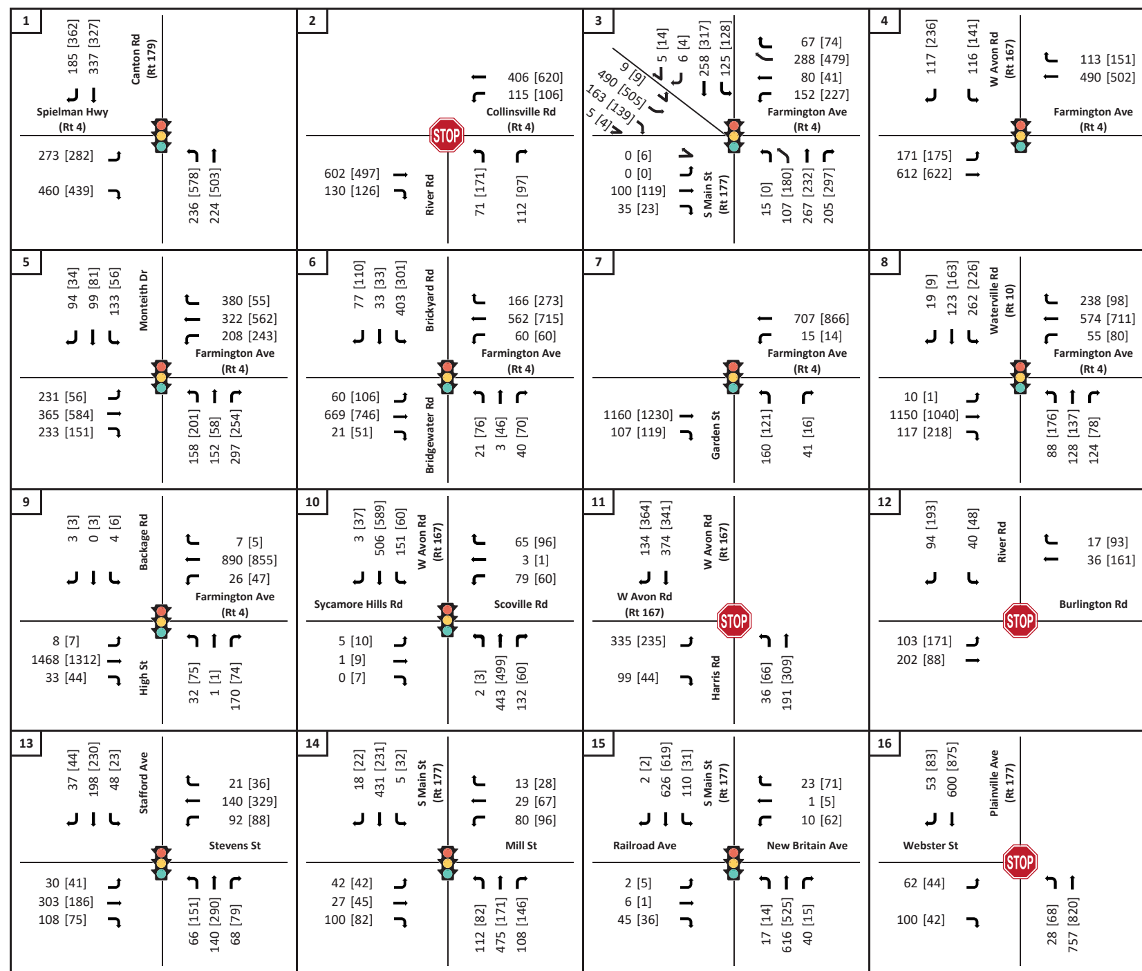
Figure 10a - Scenario 2 (2050 Build Conditions) Peak-Hour Traffic Volumes (Intersections 1-16)
